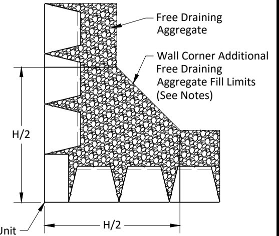
Typical 2nd and / or Even Numbered Courses Plan
