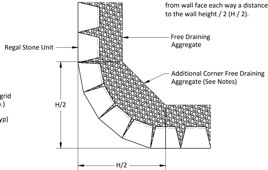
Typical Outside Curve Plan
