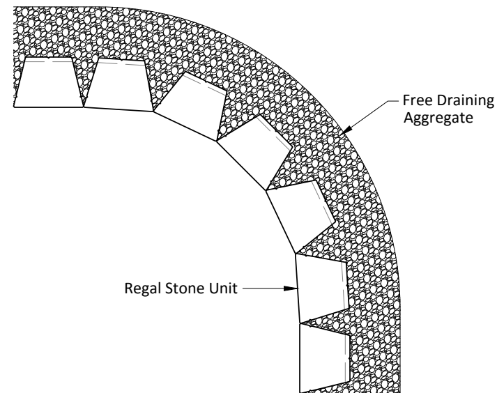
Typical Inside Curve Plan
