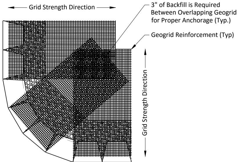
Outside Curve Plan with Geogrid
