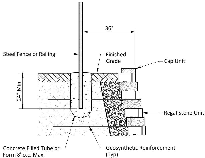
Fence Section
