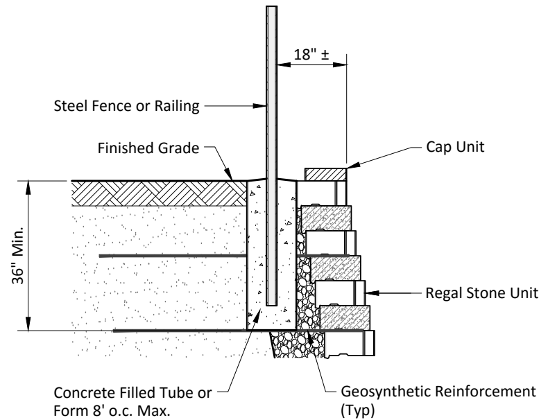
Minimum Offset Fence Section
