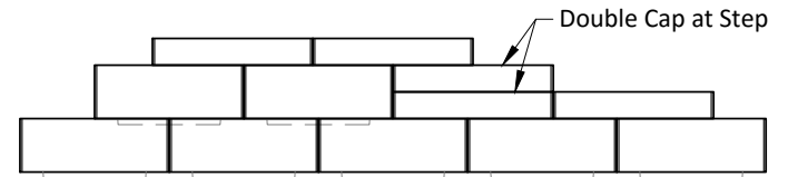
Cap Units Wall Step Plan
