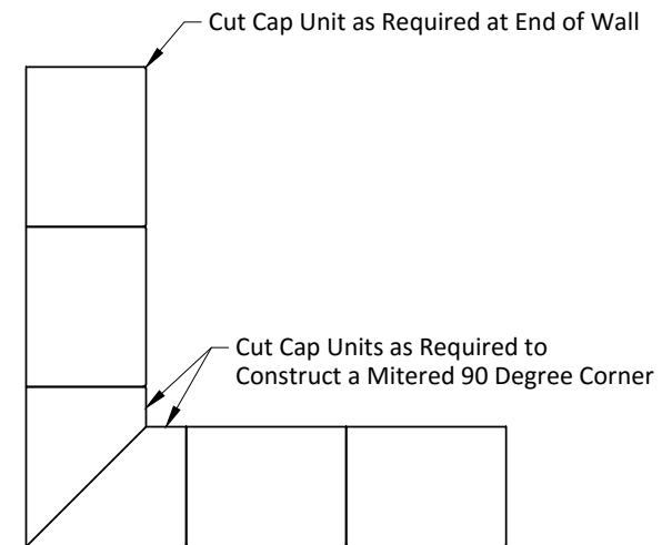
Cap Units Corner / Wall
