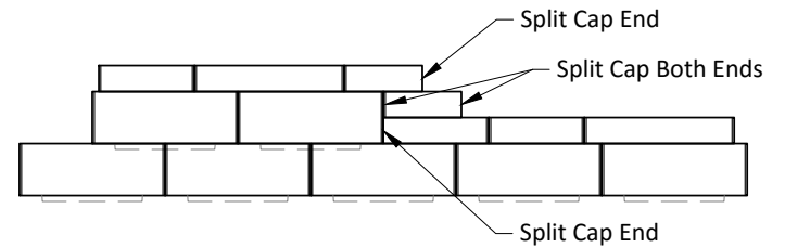
Cap Units Wall Step Plan
