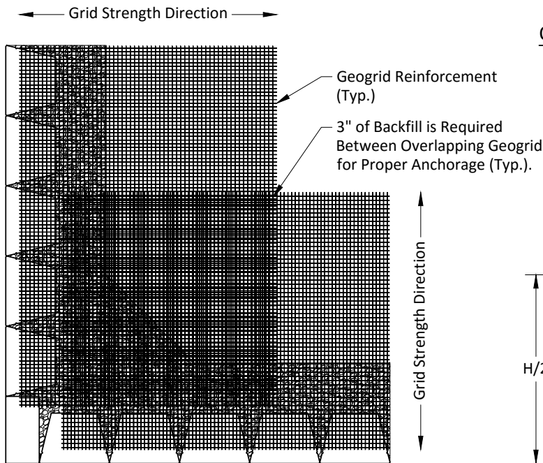
Outside Corner Plan with Geogrid
