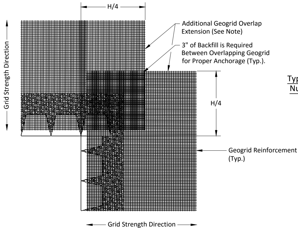
Inside Corner Plan with Geogrid
