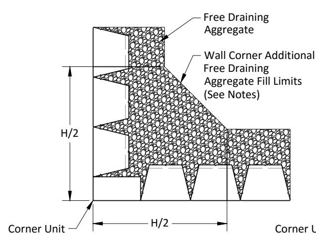
Typical Base and / or Odd Numbered Courses Plan
