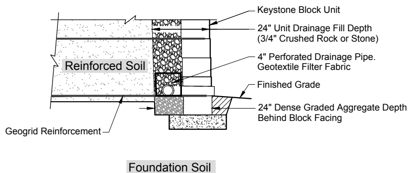
E:5 - ALTERNATE RAISED DRAINAGE PIPE LOCATIONS
