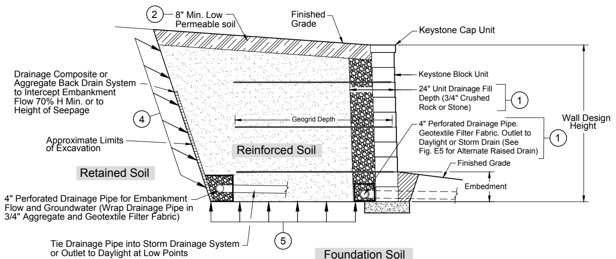
E:3 - TYPICAL DRAINAGE WALL SECTION
