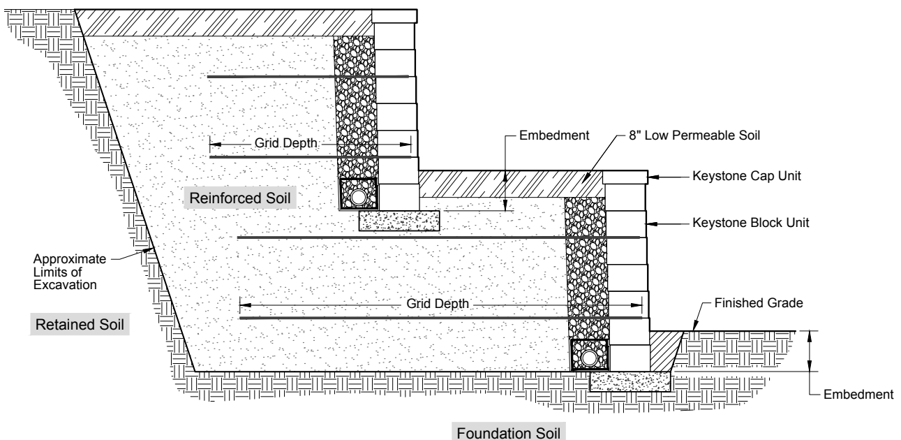
E:12 - TIERED REINFORCED WALL
