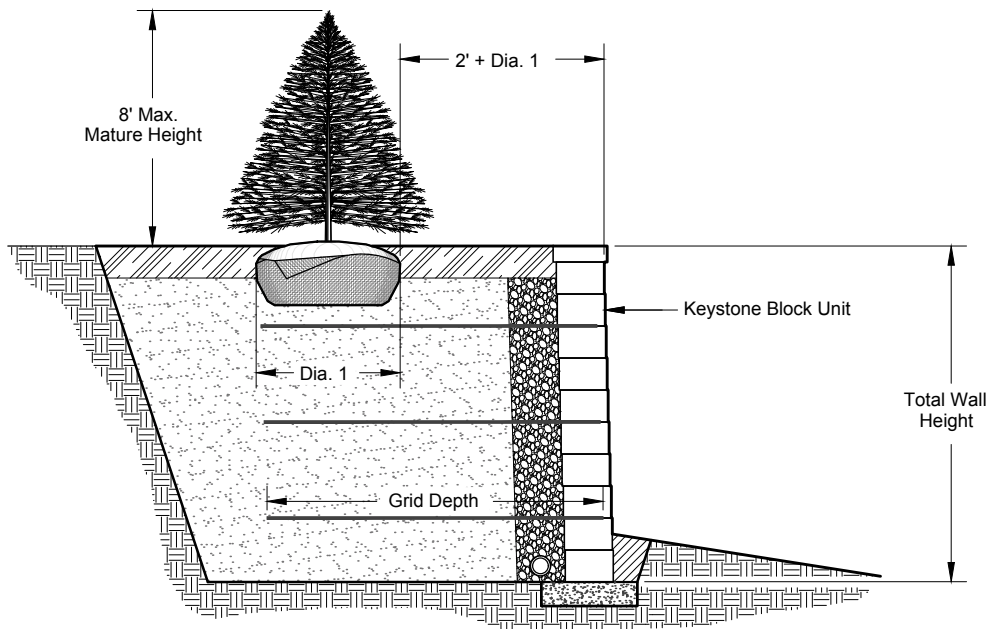
E:13 - PLANTING LIMITS BEHIND WALL
