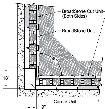
C:2 - TYPICAL SECOND: EVEN COURSES
