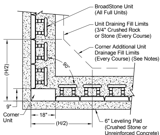
C:1 - OUTSIDE CORNER: ODD COURSE
