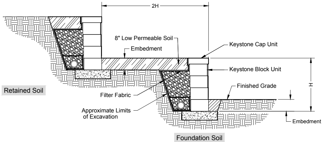
E:11 - INDEPENDENT TIERED GRAVITY WALL
