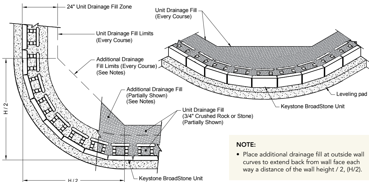
C:16 - OUTSIDE CURVE ADDITIONAL DRAINAGE FILL
