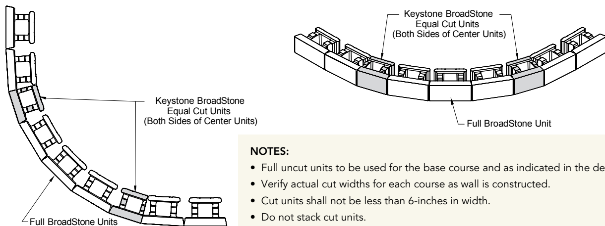
C:15 - OUTSIDE CURVE RUNNING BOND
