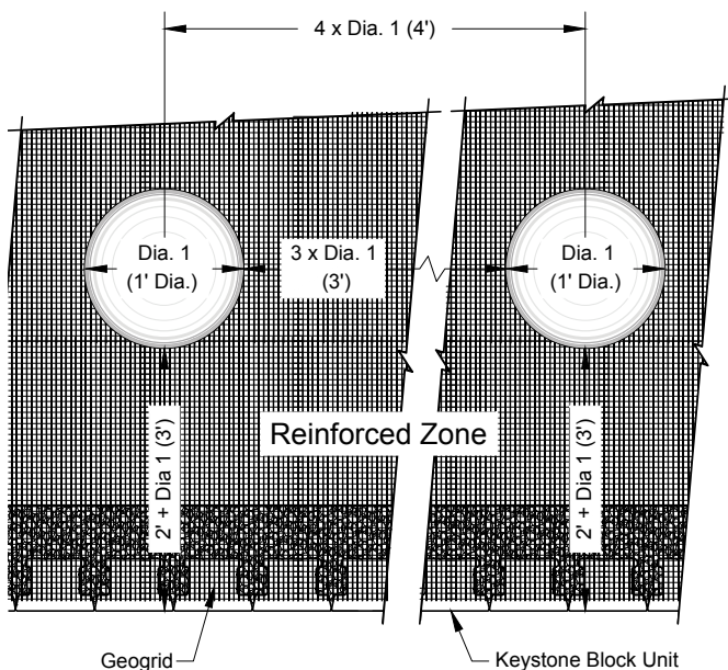
E:14 - PLANTING LIMITS BEHIND WALL
