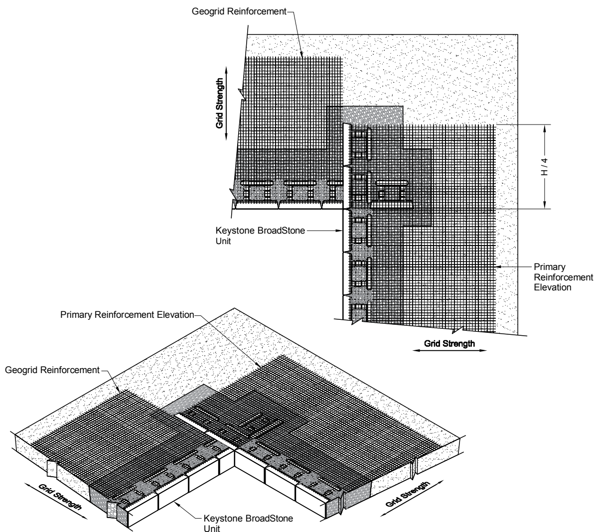
C:9 - TYPICAL GEOGRID INSTALLATION FOR INSIDE CORNERS
