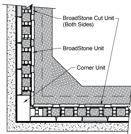
C:3 - CORNER PLAN VIEW
